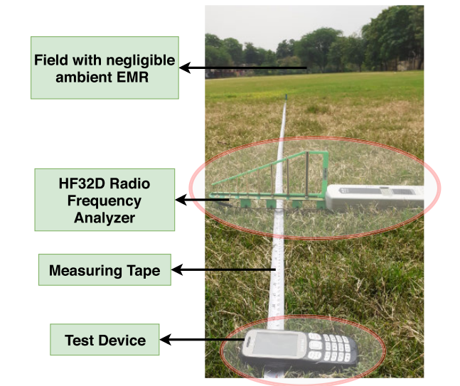
FIGURE 4. The location for testing was an open field with ambient Power Flux Density less than 5 \mu W/m^2 .
