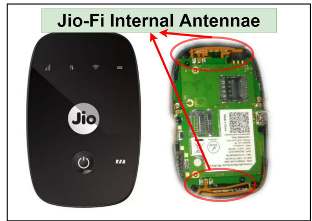
(b) Antennas in a portable Wi-Fi router
