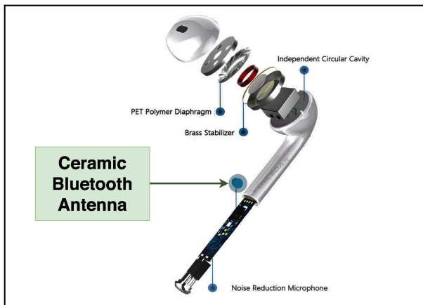
(c) Antennas in Bluetooth earphones
